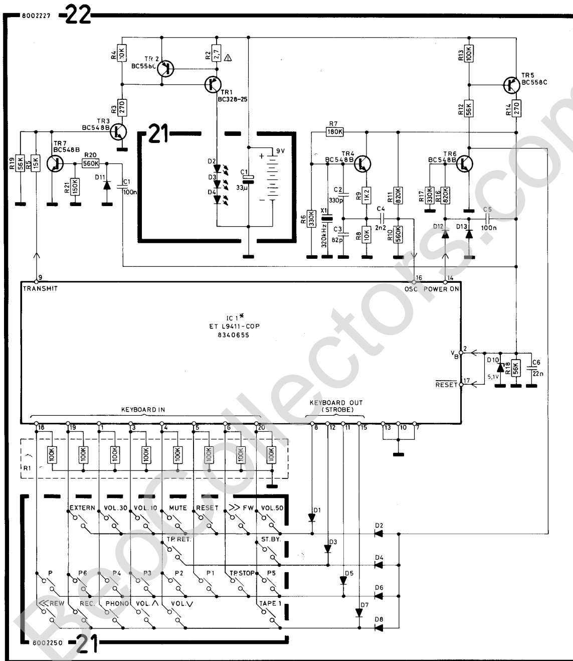
DIAGRAM 4 FOR BEOMASTER TERMINAL TYPE 2035 (Based on IC - 8340655)
